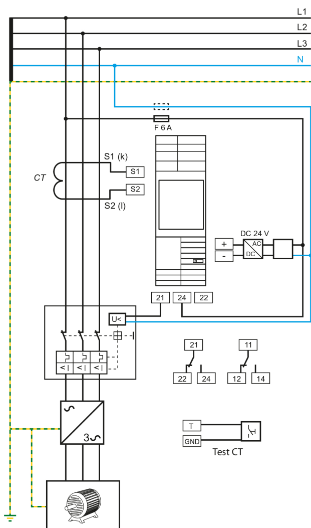
Wiring diagram for undervoltage release
